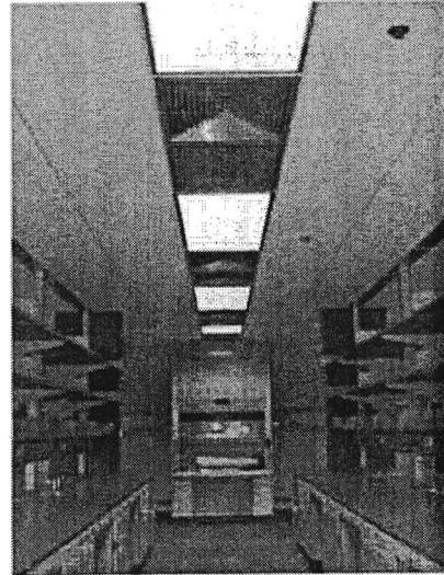
Lab Work
